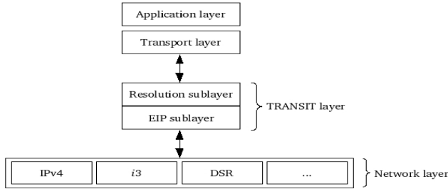
Figure 2: A network layer agnostic, TRANSIT-enabled TCP/IP stack.
